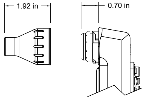
Nozzle and Diffuser
