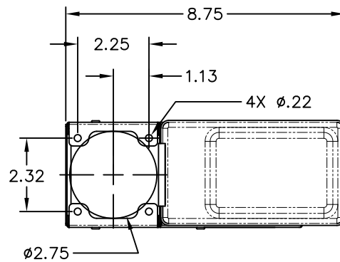
MOUNTING DETAIL:
