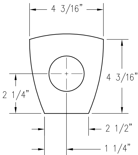
RUBBER GASKET
